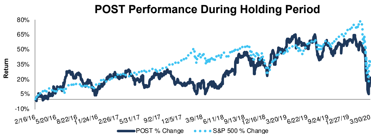
Figure 1: POST vs. S&P 500 – Price Return – Successful Short Call
