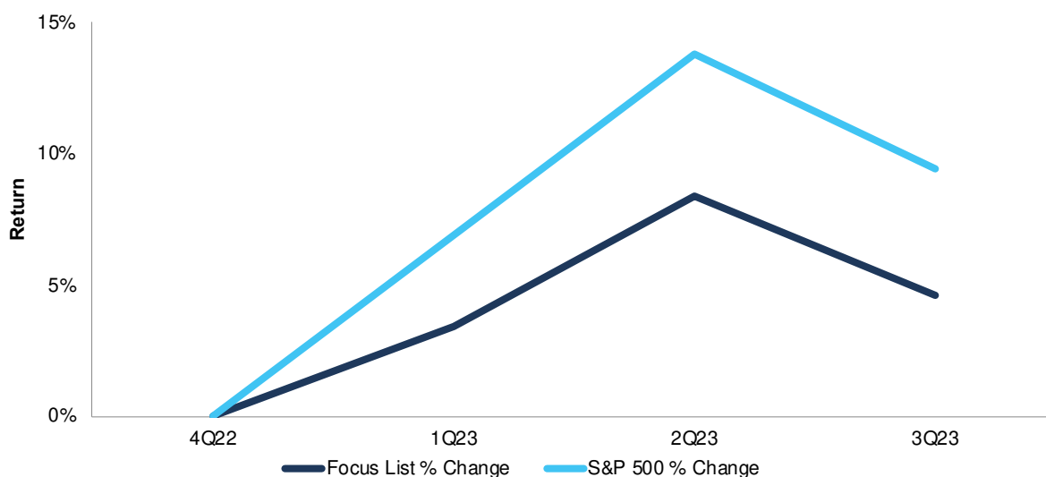
Figure 1: Focus List Stocks: Long vs. S&P 500 in First Nine Months 2023
